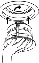
Figure 2 Connect the wires and place the speaker in the frame, twist and lock.
