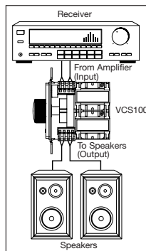
Figure 3 Wiring Diagram
